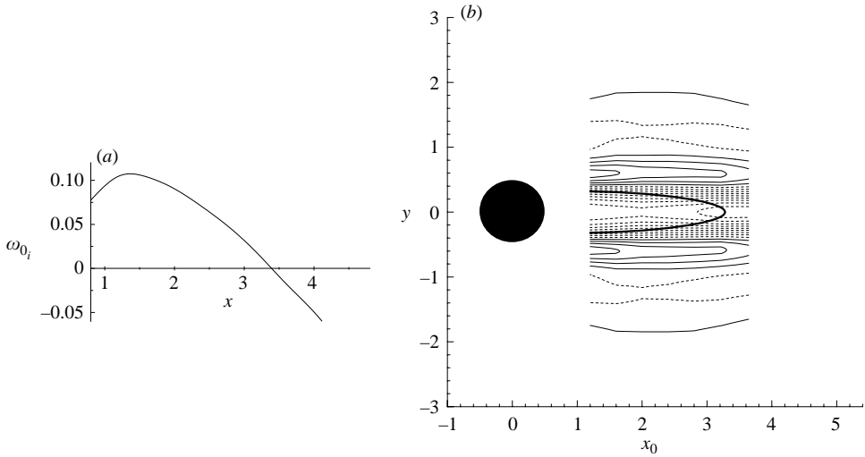
FIGURE 3. Distributions of the local absolute-instability frequency and sensitivity function in the streamwise direction (circular-cylinder wake at Re_D = 48 ): (a) \omega_{0,i}(x) ; (b) K_{0,i}(y; x_0) . In (b), the solid and dashed lines denote, respectively, positive and negative values ( -1.8 to 0.6 in increments of 0.2 ), and the thick solid line denotes the contour of U = 0 .
